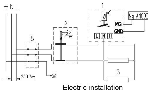
Electric installation
